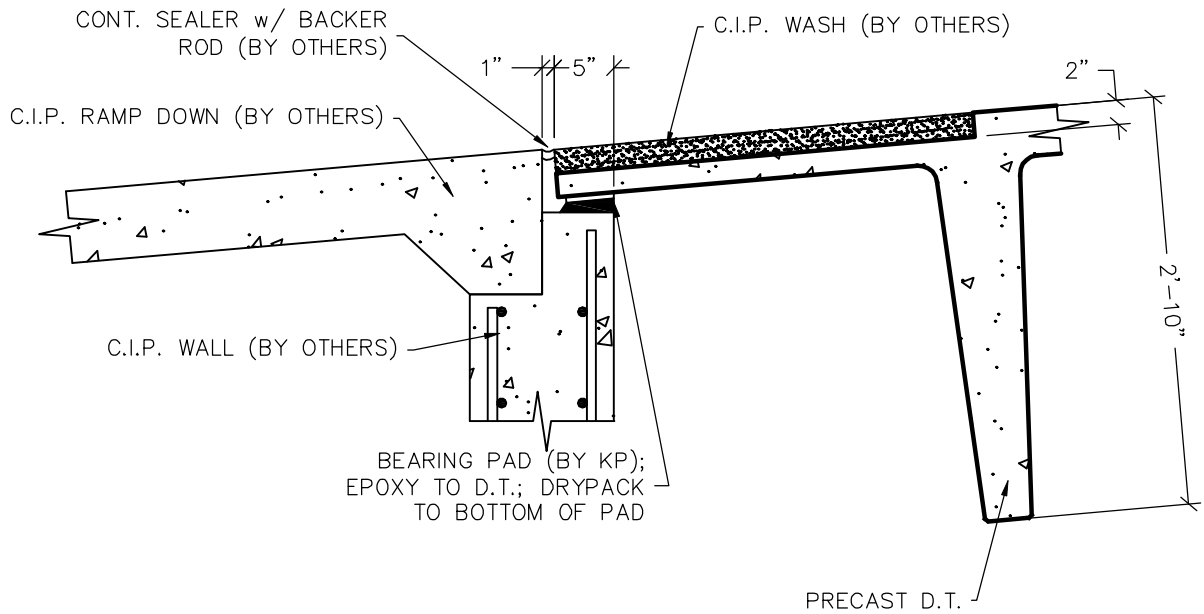
1 SECTION 12 \frac{3}{4}'' = 1'-0''
