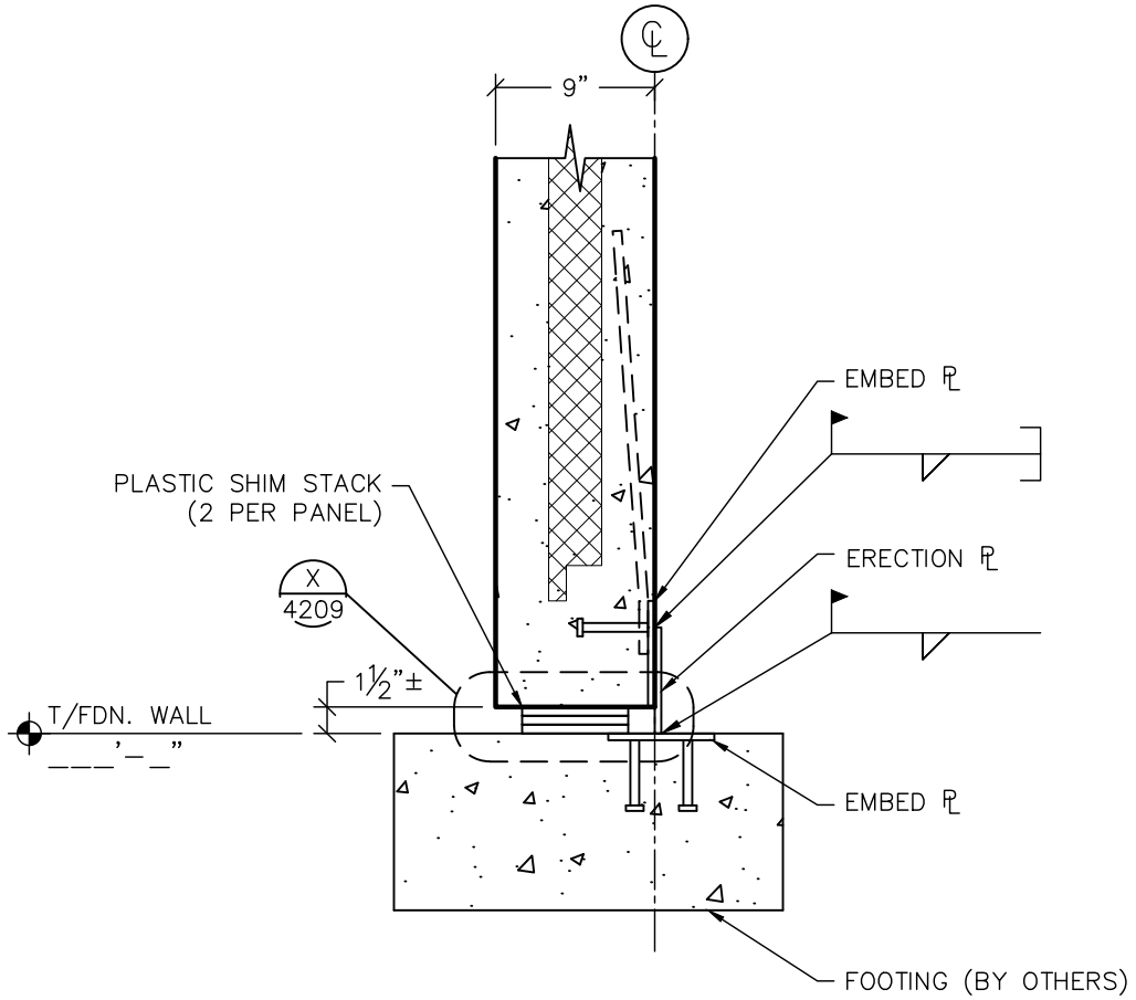
SECTION 1" = 1'-0"
