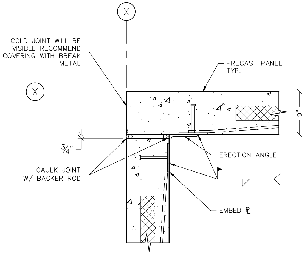
SECTION 1" = 1'-0"
