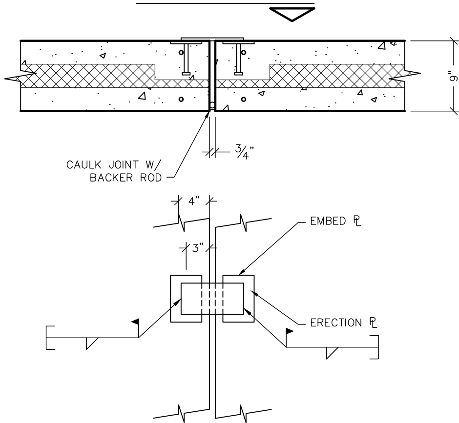
SECTION 1" = 1'-0"
