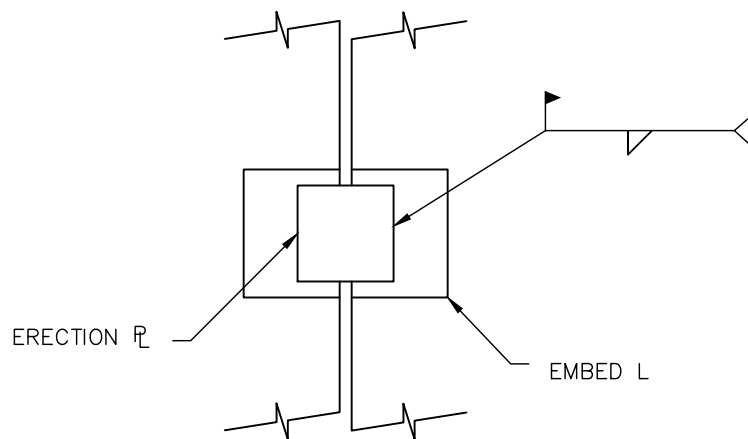
SECTION 1" = 1'-0"
