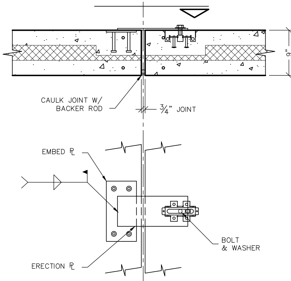
SECTION 1" = 1'-0"
