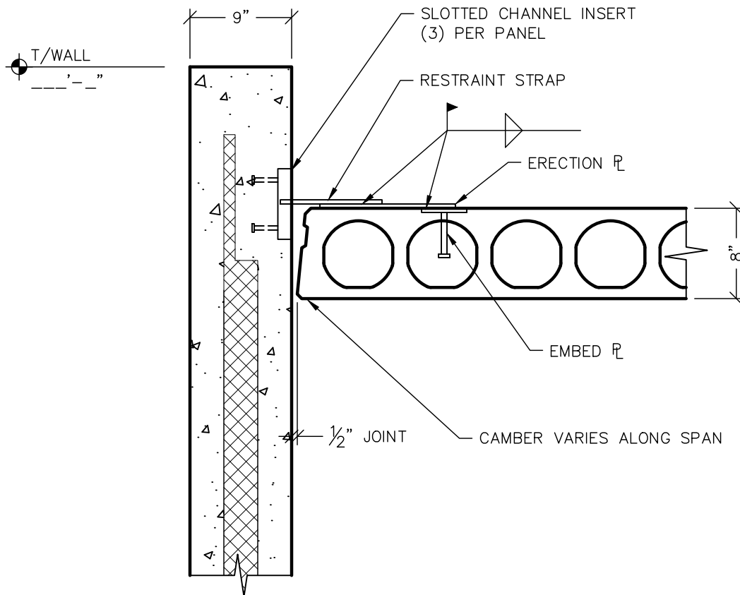
SECTION 1" = 1'-0"
