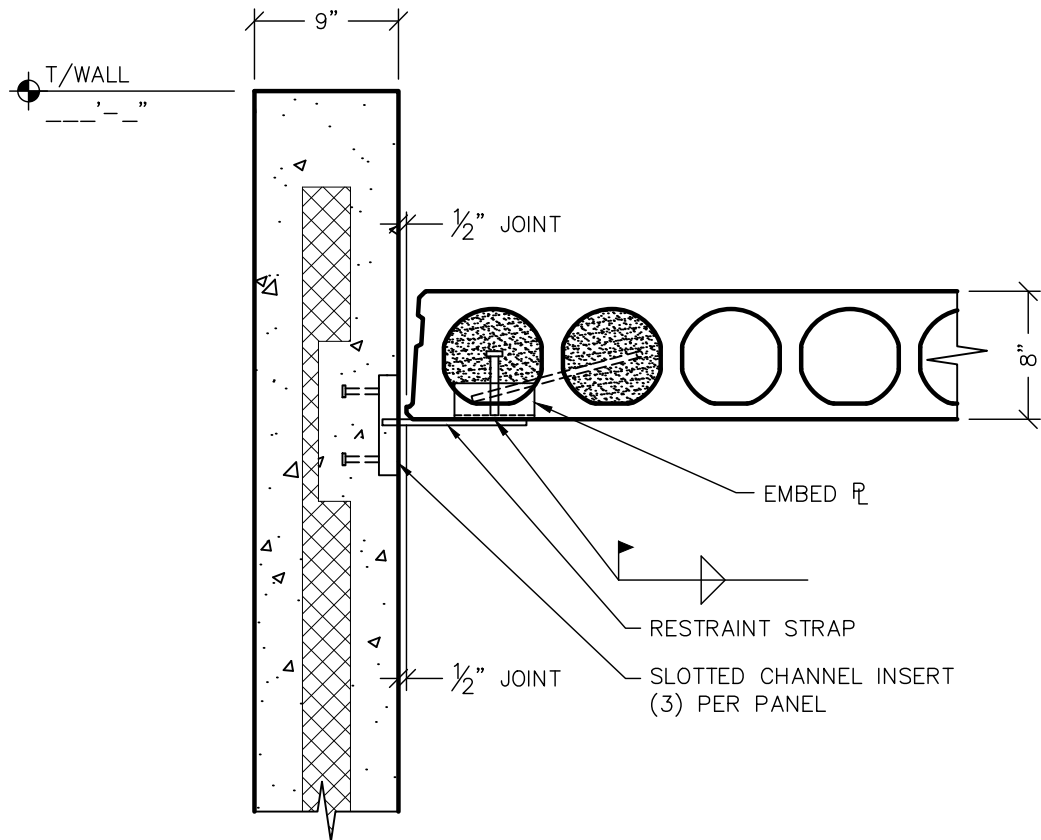
SECTION 1" = 1'-0"
