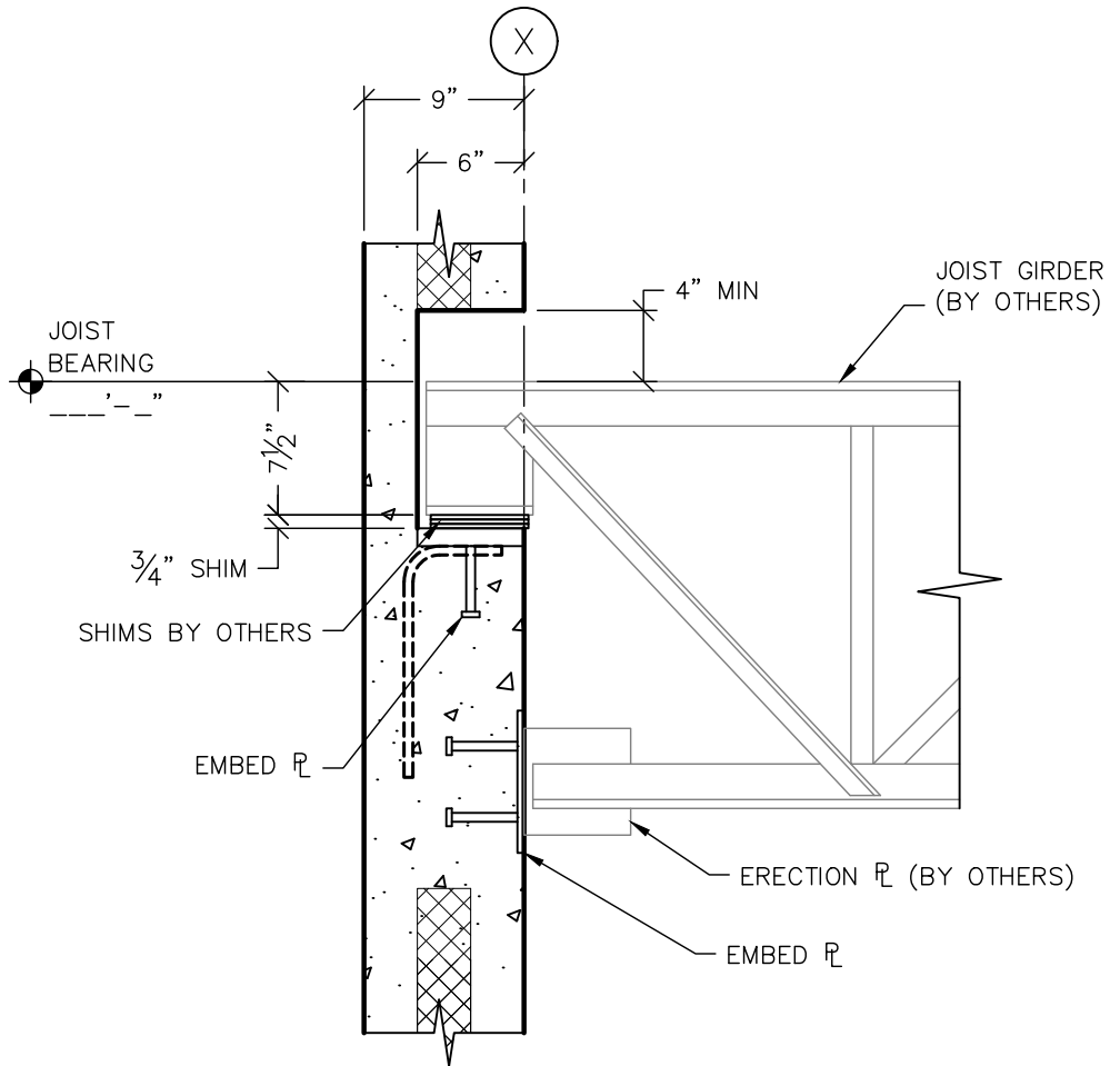
SECTION 1" = 1'-0"
