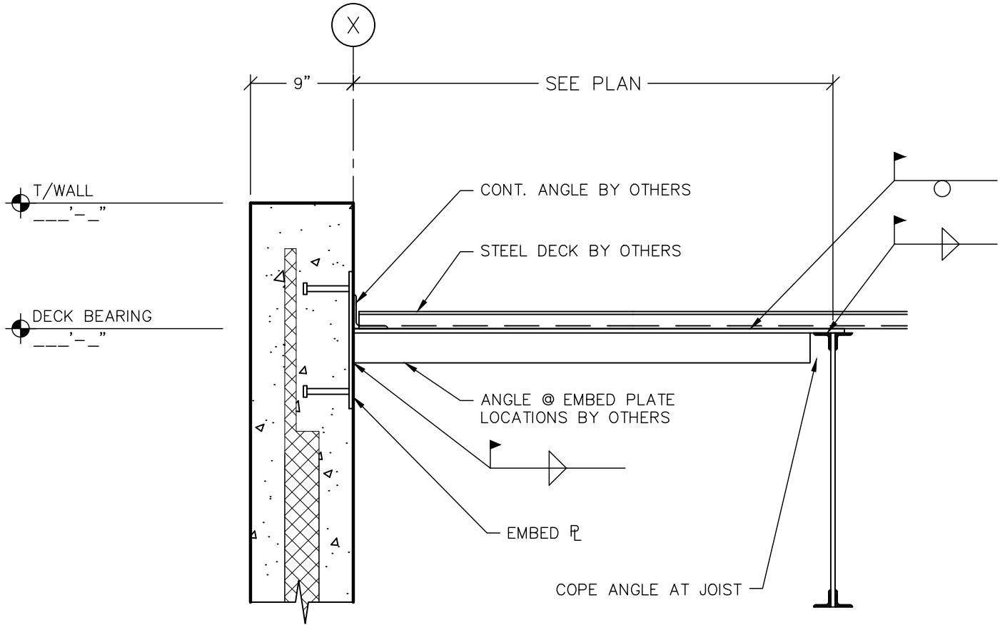
SECTION 1" = 1'-0"
