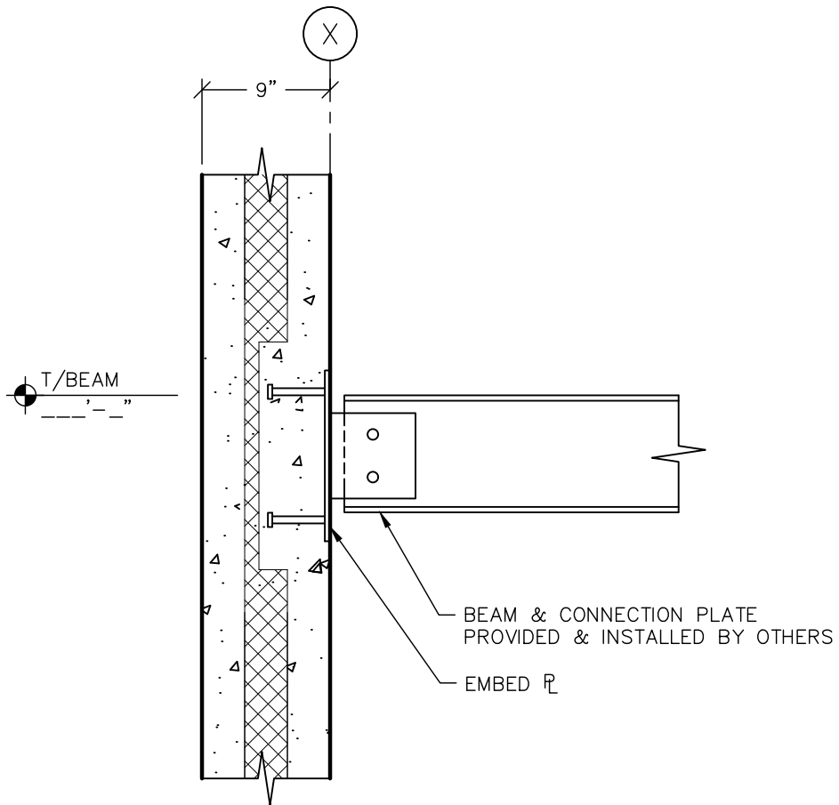
SECTION 1" = 1'-0"
