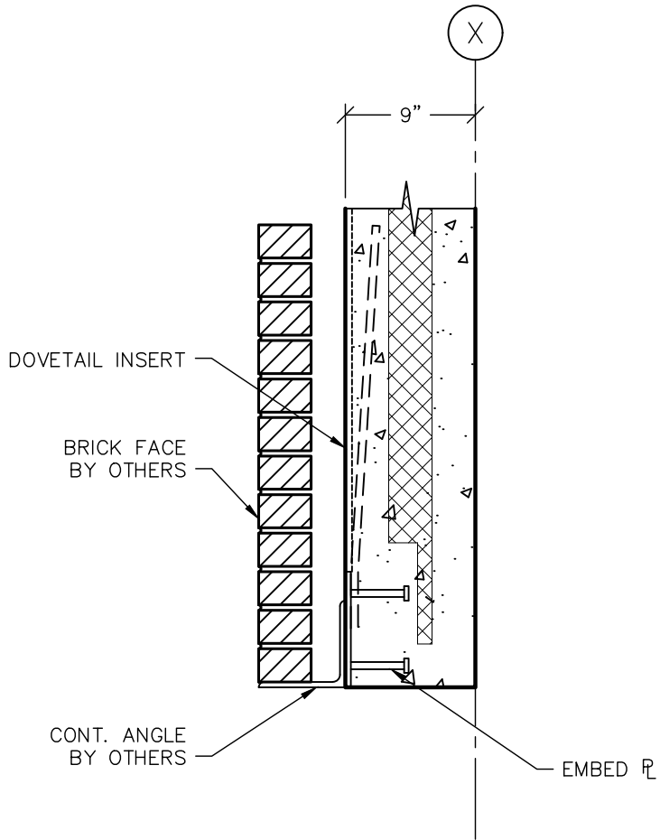
SECTION 1" = 1'-0"
