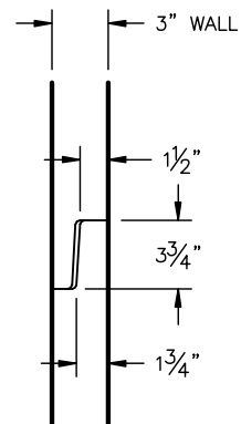
3" WALL
