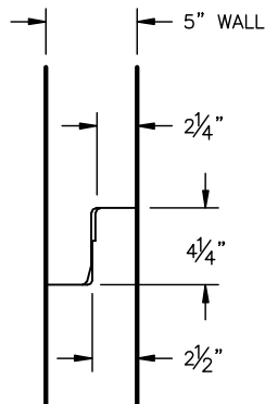
SINGLE OFF SET SANITARY & STORM 48" DIA. MANHOLE
