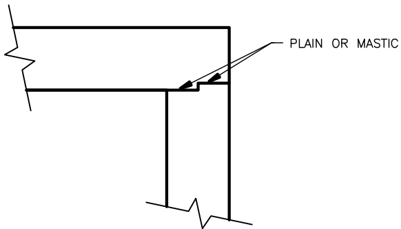
TONGUE & GROOVED JOINT CONNECTION
