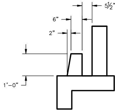
BAFFLE DETAIL
