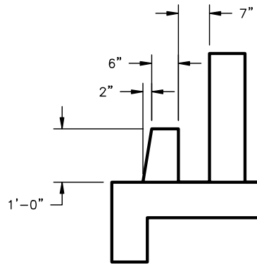
BAFFLE DETAIL
