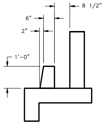
BAFFLE DETAIL
