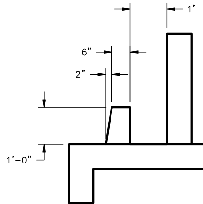
BAFFLE DETAIL
