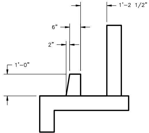
BAFFLE DETAIL
