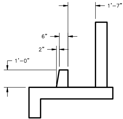
BAFFLE DETAIL
