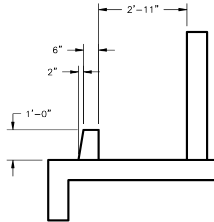
BAFFLE DETAIL
