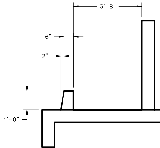
BAFFLE DETAIL
