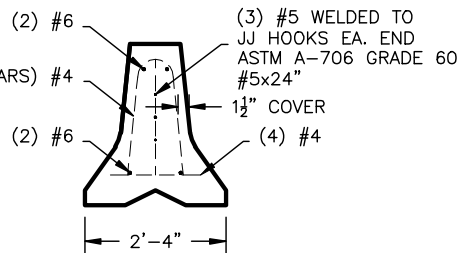
REINFORCING SECTION
