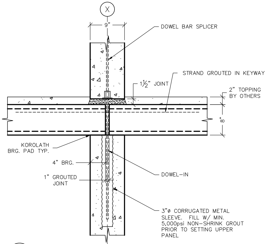
SECTION 1" = 1'-0"
