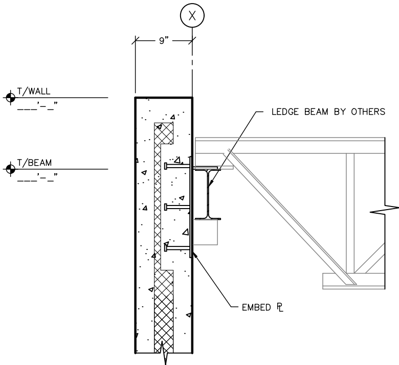
SECTION 1" = 1'-0"
