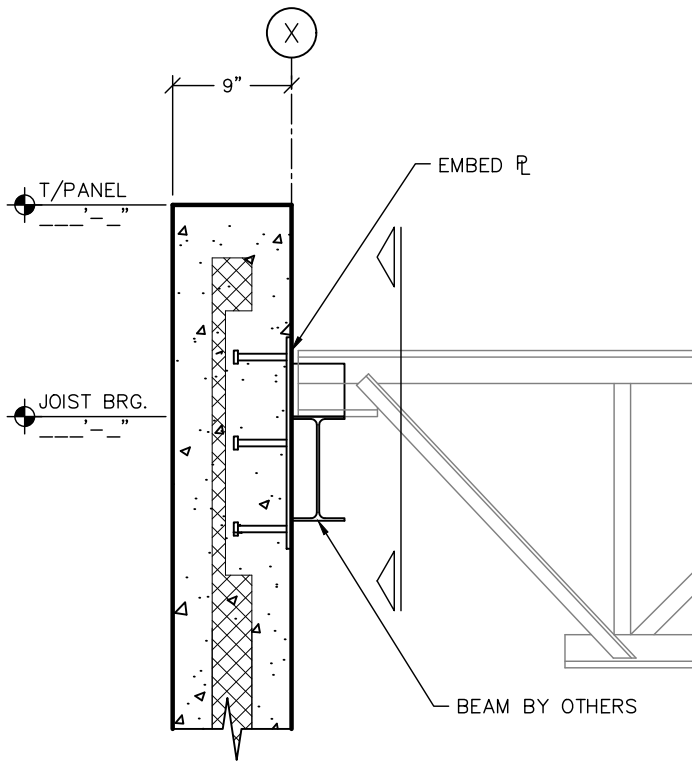
SECTION 1" = 1'-0"
