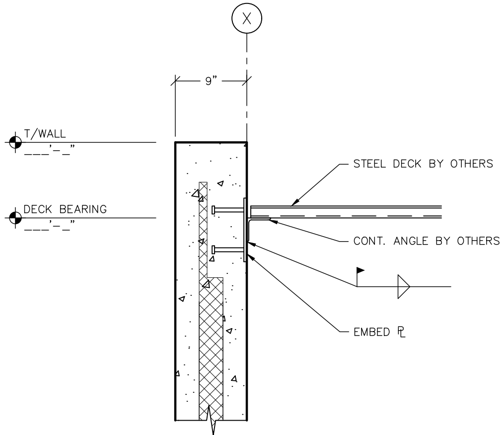
SECTION 1" = 1'-0"
